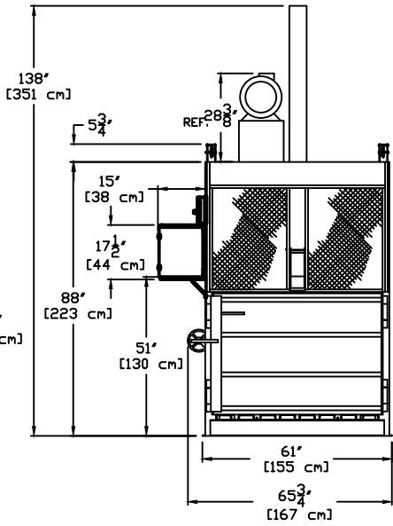
FRONT VIEW HINGED RIGHT SIDE
