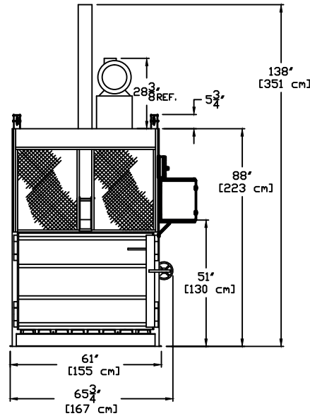
FRONT VIEW HINGED LEFT SIDE
