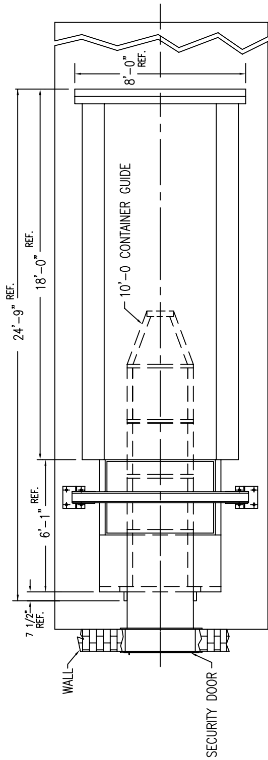
TOP VIEW
